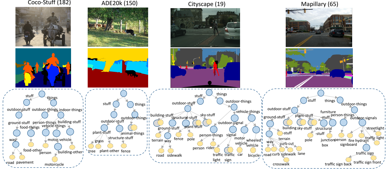
Figure 3. DSSPN can learn a unified segmentation model for accommodating diverse annotation policies. For training with diverse annotations with discrepant label granularity, DSSPN activates dynamic-structured semantic propagation graphs for each image. For example, Ade20k only annotates a single “animal-thing” label for all animal categories while Cocostuff elaborately categories each fine-grained concept, e.g. cat or elephant. The semantic neurons that correspond to target labels are deactivated (grey colored solid circles). It thus fully exploits the shared concept patterns and concept relationship in a semantic hierarchy for a more general segmentation model. For simplicity, only target labels and their ancestor concepts are shown.
