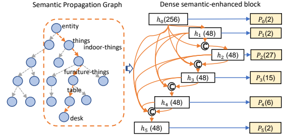
Figure 2. Dense semantic-enhanced block. For each activated semantic neuron v_i , it concatenates features evolved from the neurons in the whole path (dashed orange arrows) to obtain enhanced representation h_i , which is further passed through dynamic pixel-wise prediction P_i for distinguishing between its children nodes. The output dimensions (e.g. 48) of each block and those (e.g. 27) of pixel-wise prediction layer are shown in the parentheses.
